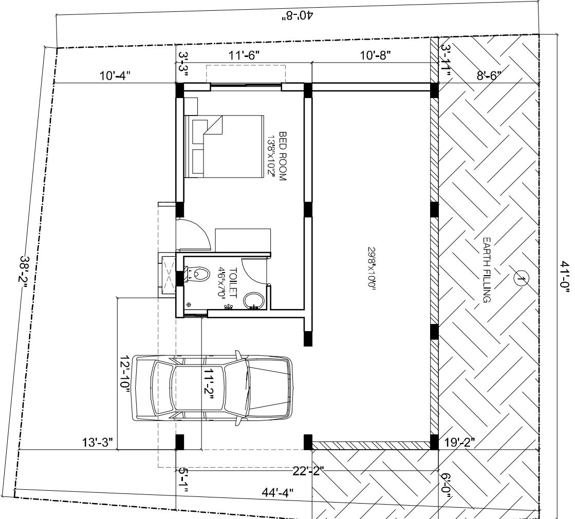
BASEMENT FLOOR
