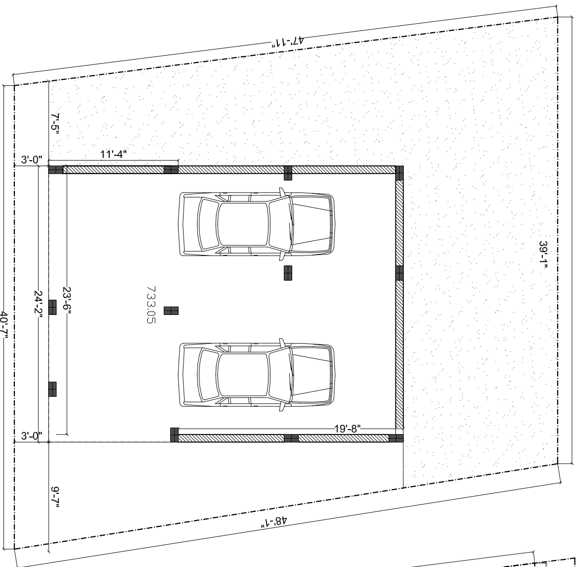
BASEMENT FLOOR
